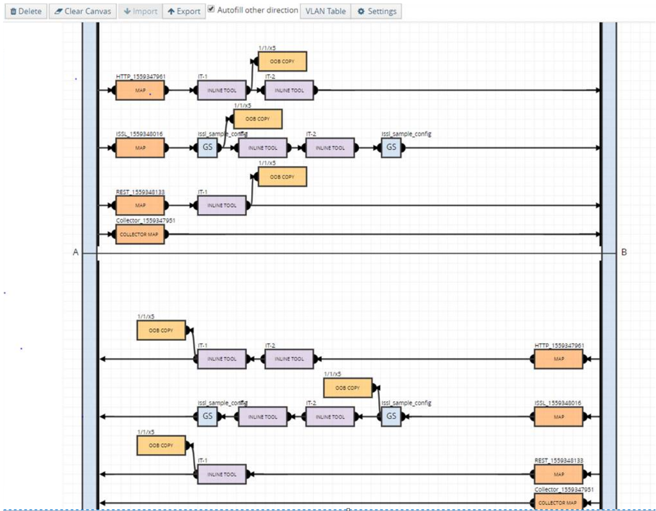
Figure 55 Flexible Inline SSL APP—Deployed
