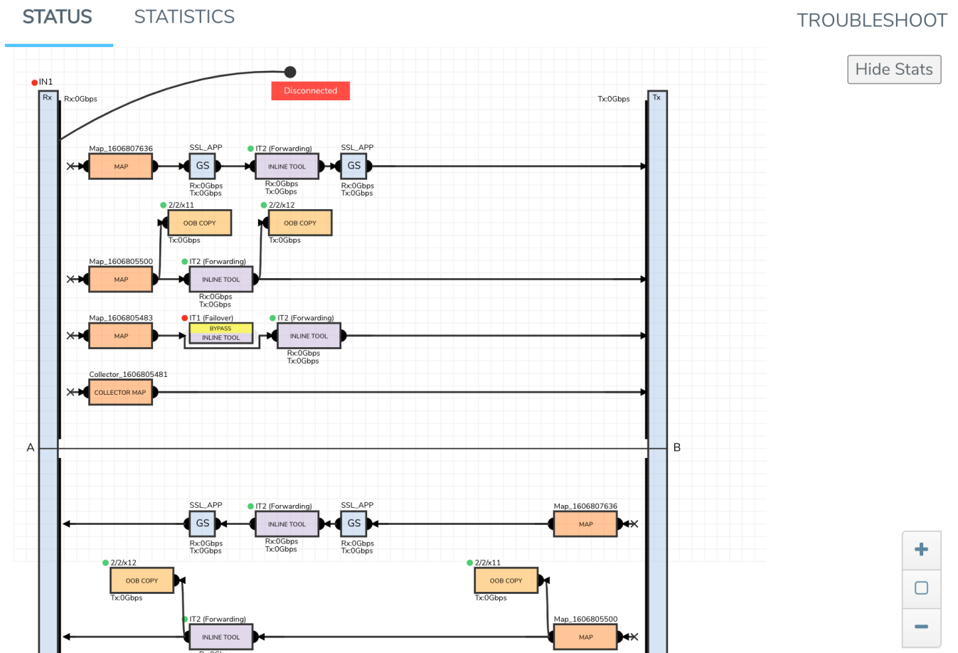
Figure 56 Inline Network Forwarding States
