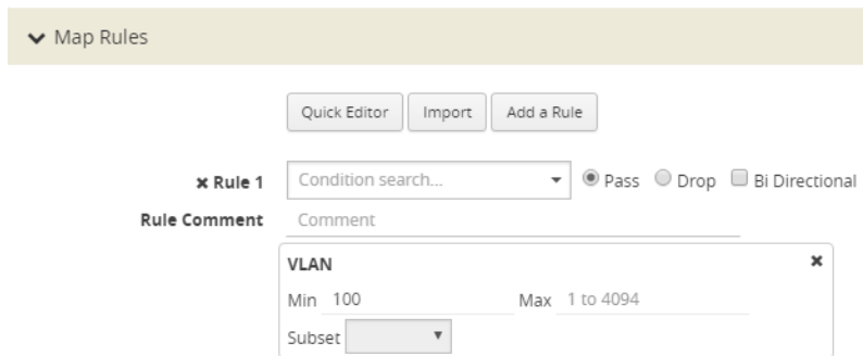
Figure 38 VLAN Pass Rule
