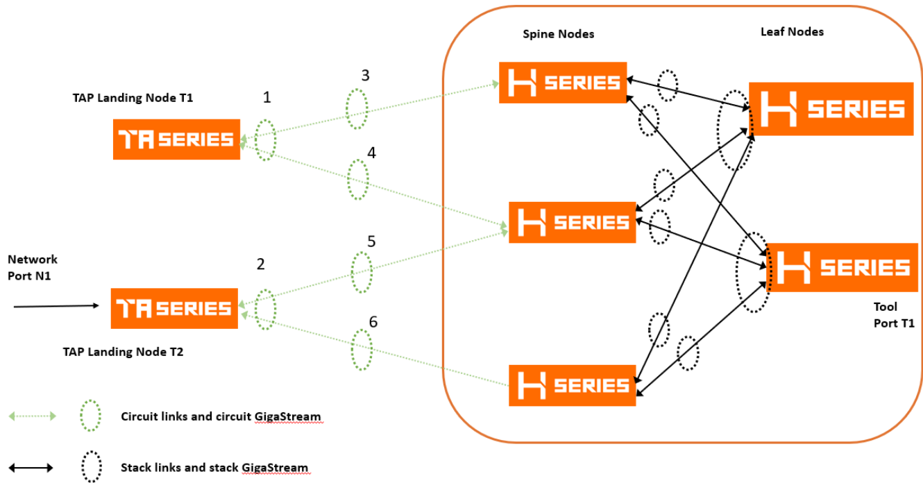
Figure 68 Leaf-Spine Based Topology.
