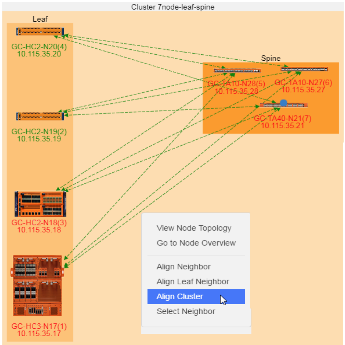
Figure 33 Displaying Align Cluster Option
