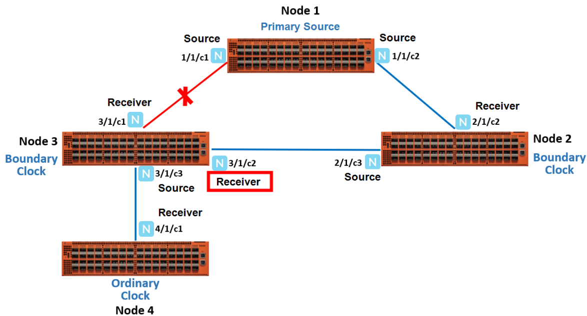
Figure 59 PTP State Transition
