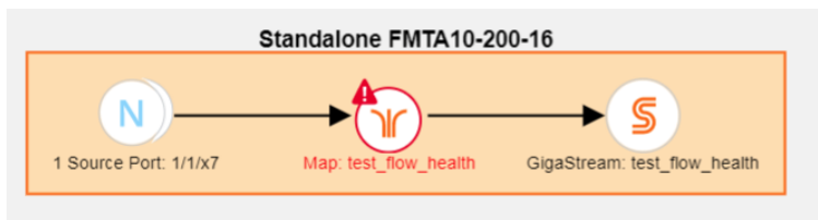
Figure 55 Unhealthy Pass-all Map
