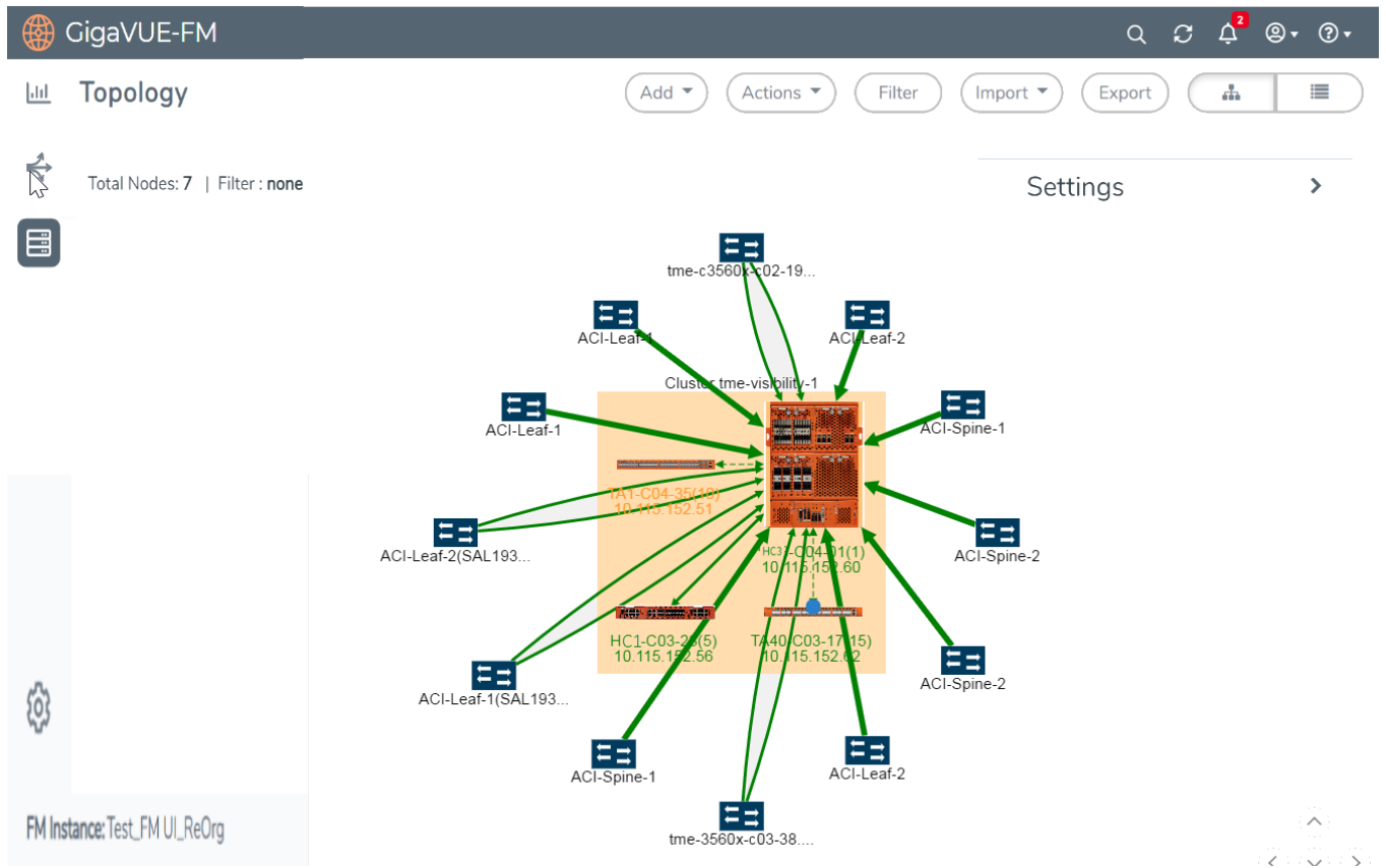
Figure 35 Physical Node Topology of a Cluster
