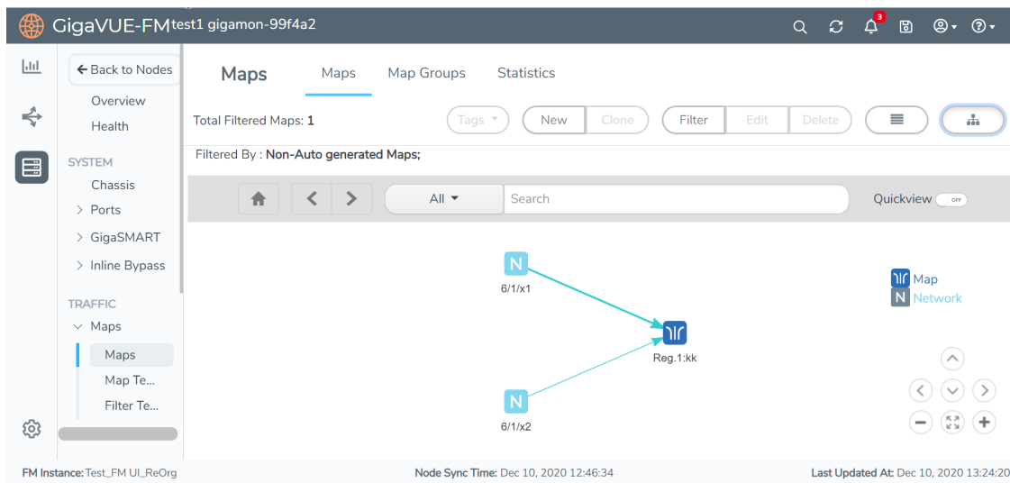
Figure 41 Map Topology View
