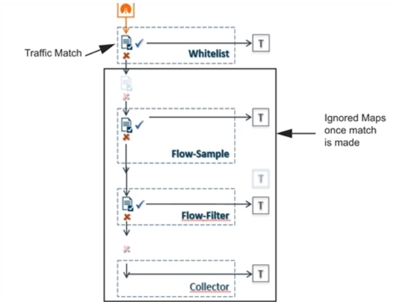
Figure 39 Non-Overlap GTP Mapping Mode
