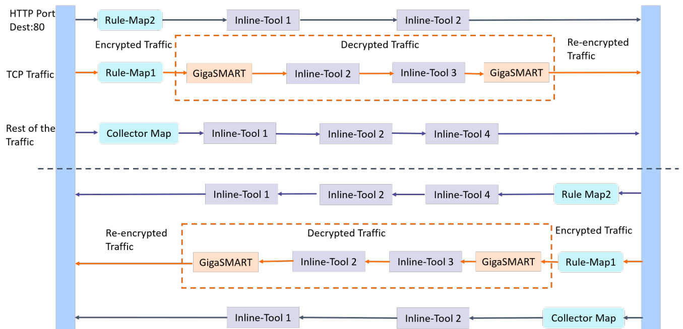
Figure 53 Flexible Inline Decryption Solution
