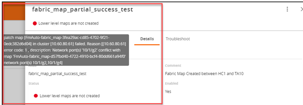
Figure 76 Fabric Maps Details
