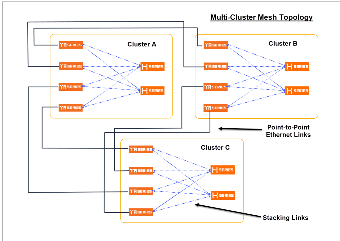
Figure 66 Multi-Cluster Mesh
