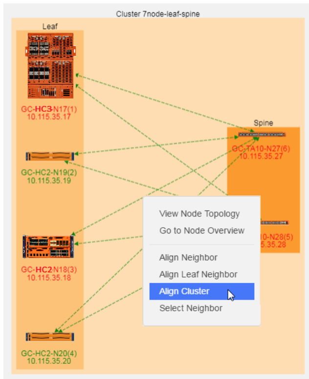
Figure 24 Context Menu Displayed for Leaf and Spine
