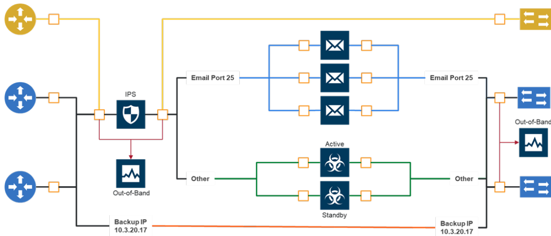
Figure 49 Flexible Inline Arrangements Scenario
