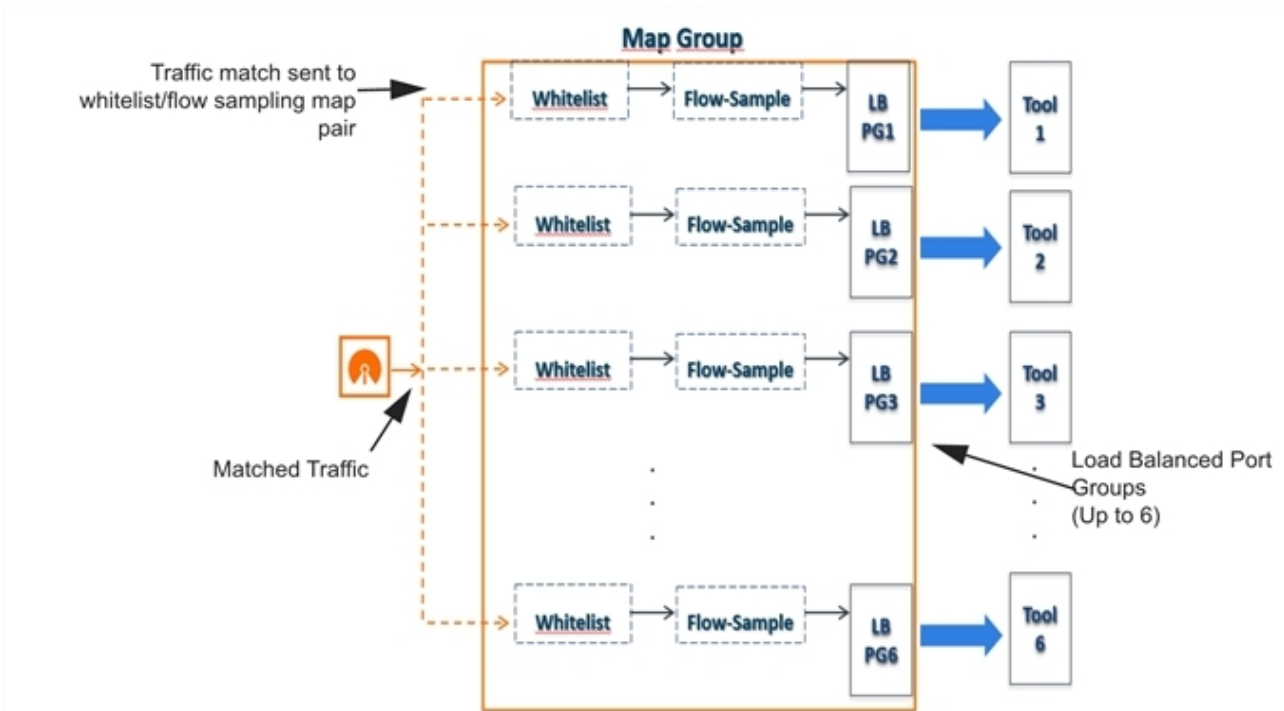
Figure 40 GTP Overlap Flow Sampling Map Groups
