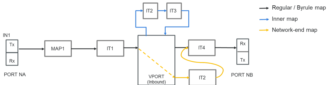
Figure 54 Flexible Inline Decryption Maps
