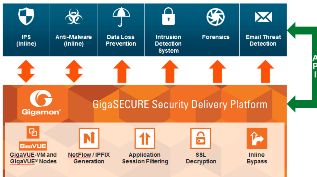
Figure 48 GigaSECURE Security Delivery Platform
