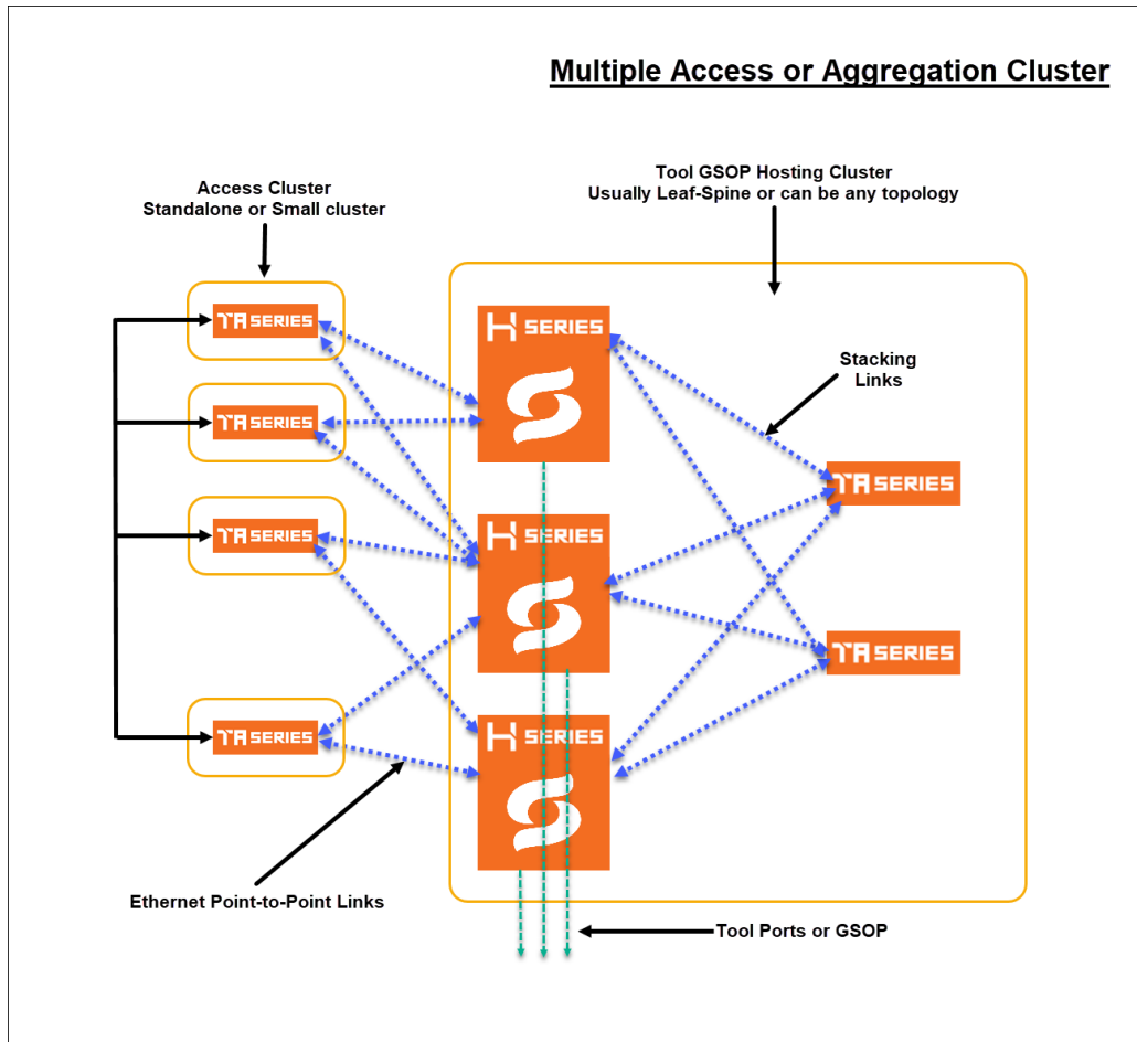
Figure 65 Multiple Access Clusters
