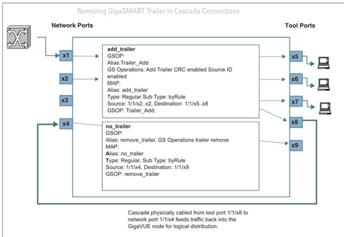
Figure 164 Removing the GigaSMART Trailer from a Cascade Connection
